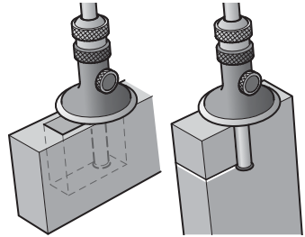
Figure 4: Transferring dimensions.
